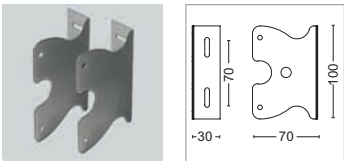
NET.AP3 07 Attacco a parete o plafone (coppia). Wall/ceiling mount (pair). Fixation plafond/mural (couple).
