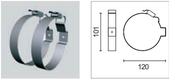
NET.AP4 Attacco a parete o plafone (coppia). Wall/ceiling mount (pair). Fixation plafond/murale (couple).
