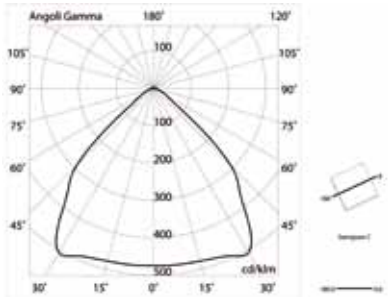
fascio 90° beam 90°
