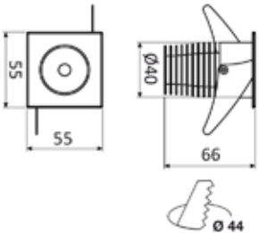
fascio 60° beam 60°
