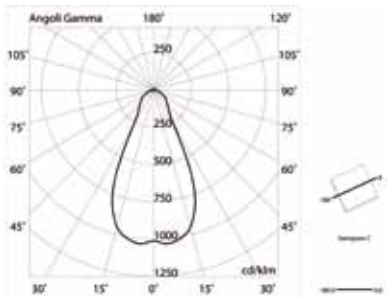
fascio 60° beam 60°
