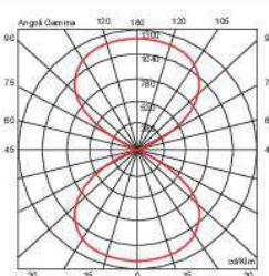
Bi-emissione a fascio largo / Double diffuse beam
